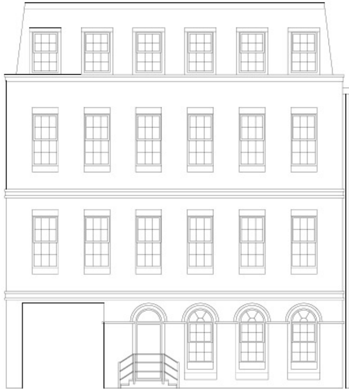
East Elevations
